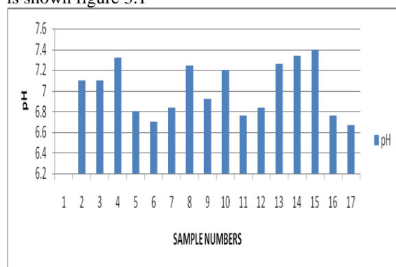
Figure 3.1: pH- Hydrogen ion concentration variations during the study period
