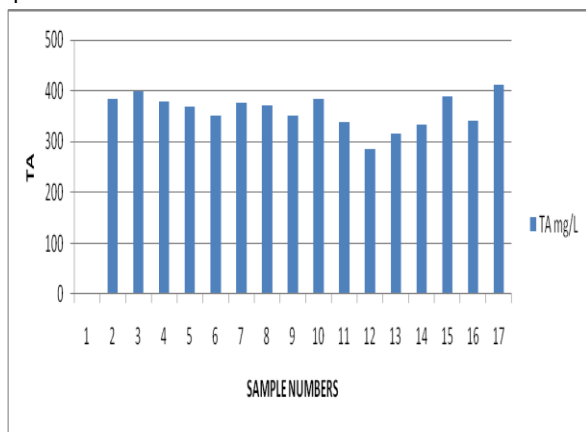
Figure 4: TH- Total Hardness, TA- Total Alkalinity variations during the study period
