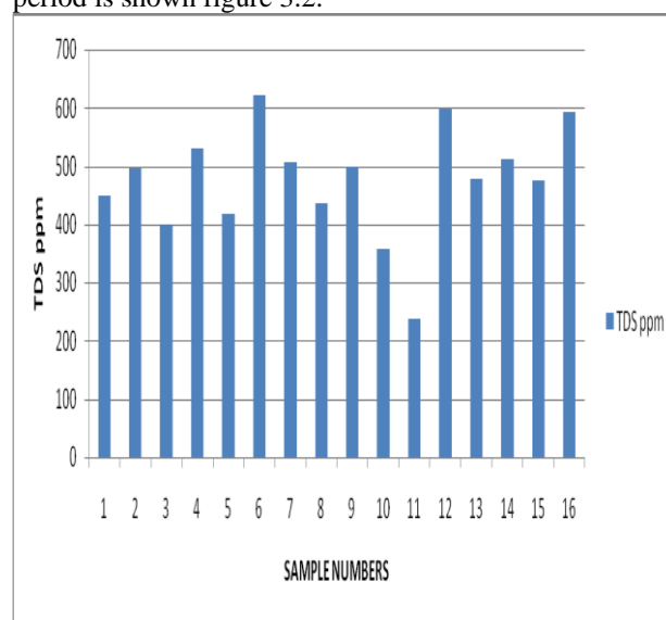
Figure 3.2: EC- Electrical conductivity, TDS- Total dissolved solids concentration variations during the study period
