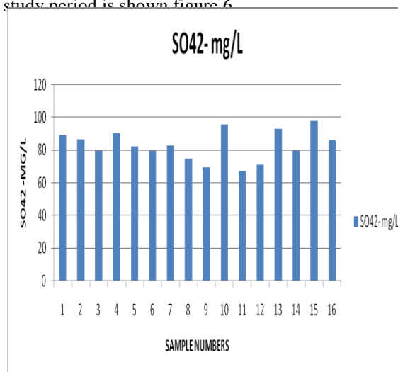
Figure 6: Cl- Chloride, SO 4 - Sulphate variations during the study period
