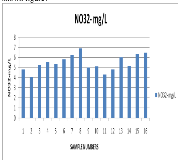
Figure 7: NO 3 - Nitrate variations during the study period
