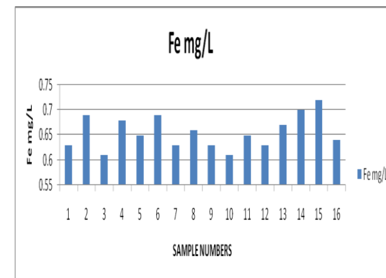
Figure 8: F- Flouride, Fe- Iron variations during study period
